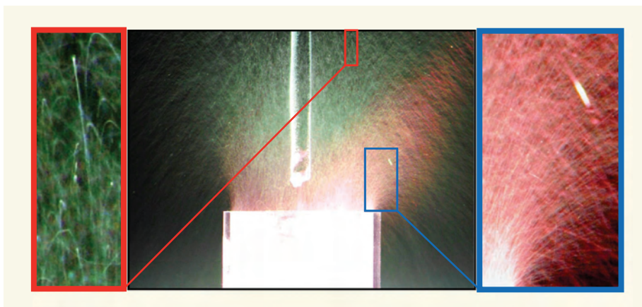
Figure 2 | Granular fountain. In this laboratory demonstration (centre) of the explosive potential of charged grains, glass beads 500 micrometres in diameter are charged by repeatedly pouring them through a vertical acrylic tube into an acrylic container. The charges on the grains become so large that the beads cannot remain at rest, and they spontaneously form a fountain that erupts from the container, even after the inflow has ceased. If the tube is electrically grounded, these ejections do not occur. Left inset, trajectories of individual grains; right inset, an apparent example of a granular aggregate coexisting alongside individual grains. Kok and Renno 1 produced a model of the development of such charge on sand. (Colours are digitally enhanced; image and experiment courtesy of F. K. Wittel, ETH-Zürich.)
